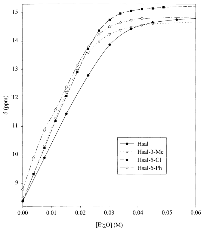
Fig. 4. A plot of \delta(-\text{CO}_2\text{H}) as a function of ether concentration for the various [\text{W}(=\text{O})\text{Cl}_3(\text{Hsal}-\text{R})]_2 compounds ( \text{R} = \text{Me}, \text{H}, \text{Ph} or \text{Cl} ).
